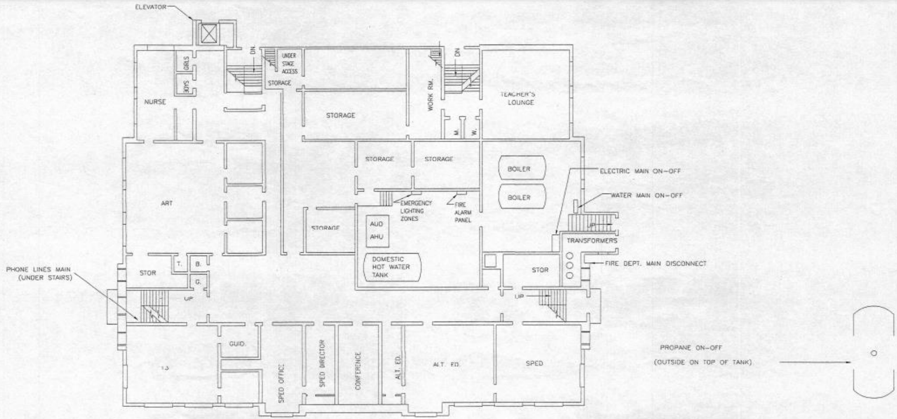
BASEMENT POWER PLAN SCALE: 1/16" = 1'-0"
